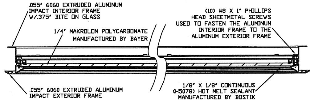
SECTION C-C SHORT PANEL IMPACT WINDOW DETAIL N.T.S.
