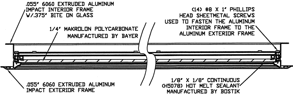
SECTION B-B LONG PANEL IMPACT WINDOW DETAIL N.T.S.
